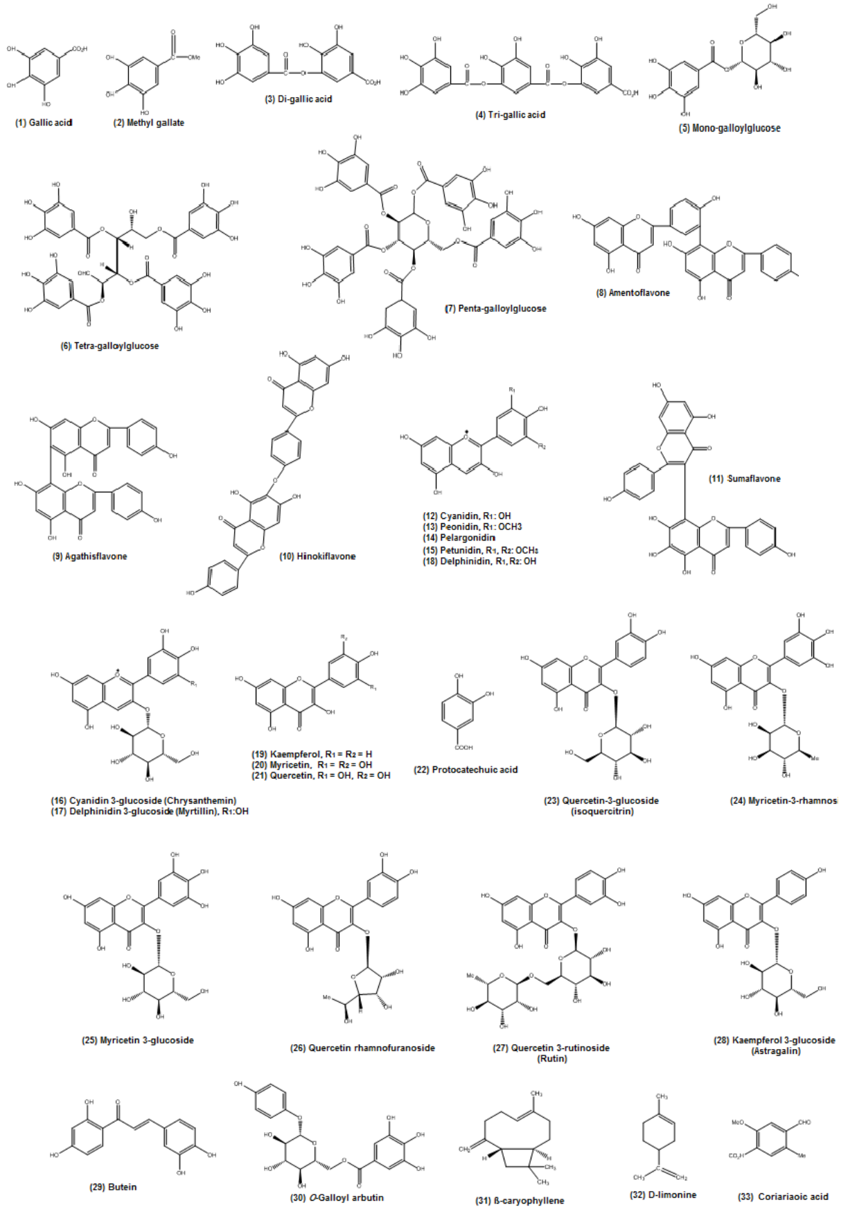
Figure 2. Structure of some selected phytochemicals from Rhus coriaria
